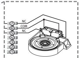
Limit Switches Connections
