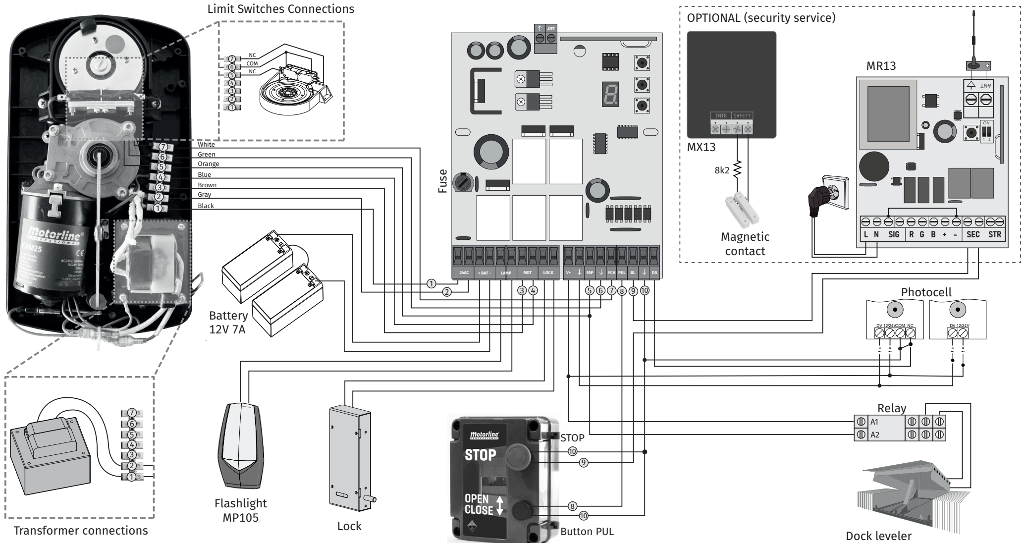
Maneuvering board
